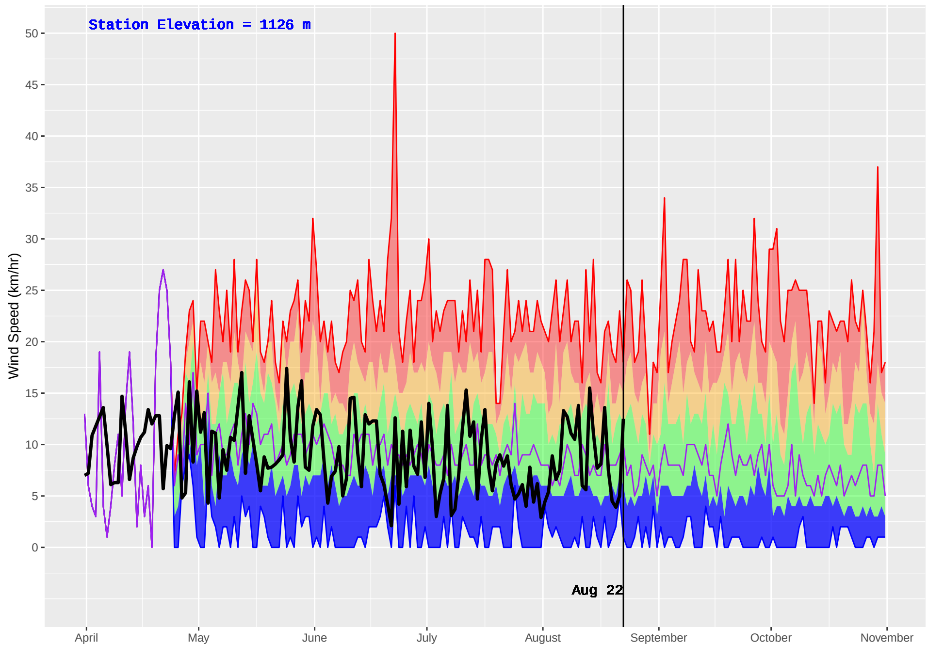
BLACKPINE (148) : Historical (1980–2016) and Current (2018) Daily Wind Speed
